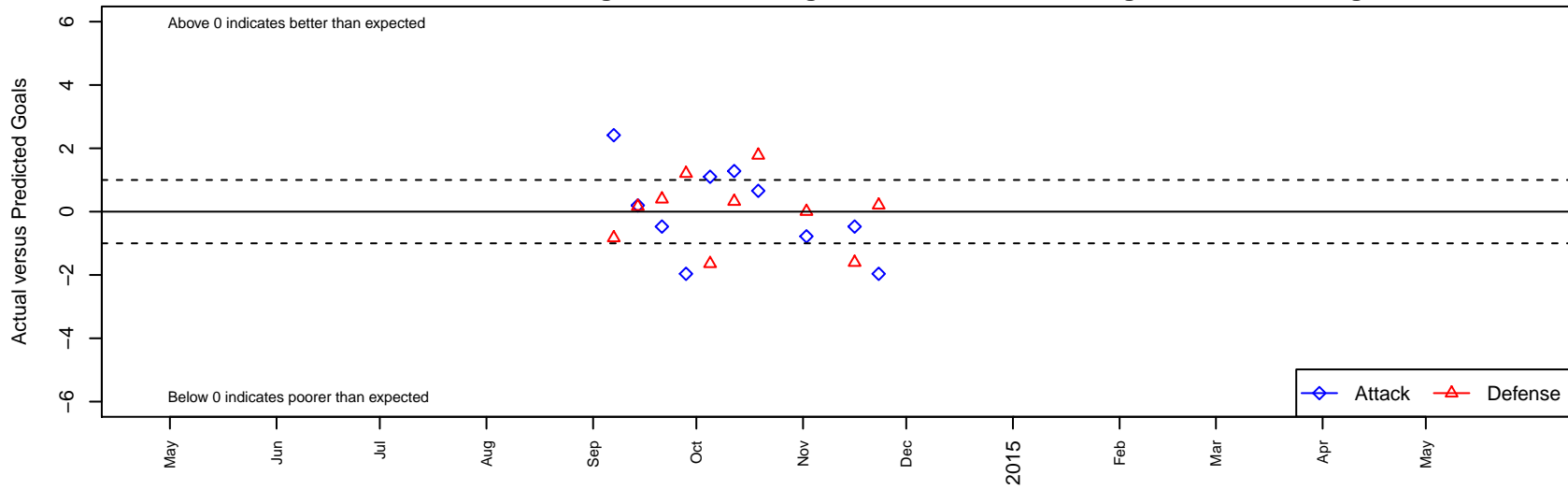
South Tacoma United Esquivel B98 Dots are actual minus expected GF (blue circles) and GA (red triangles). Blue line is smoothed change in attack strength. Red is smoothed change in defense strength.
